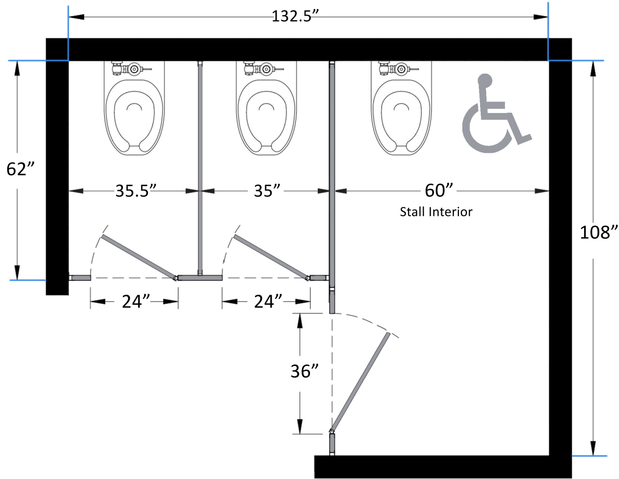
Bathroom Partitions - 3 Stall Alcove Left Hand SKU: AL3LSTD Standard Dimensions
